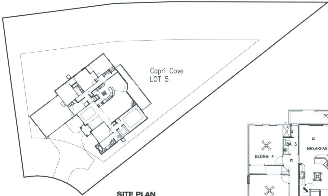
SITE PLAN
